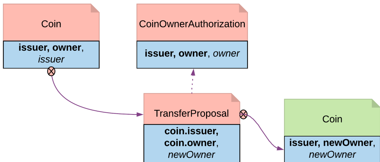
Fig. 4: Authorization Diagram
