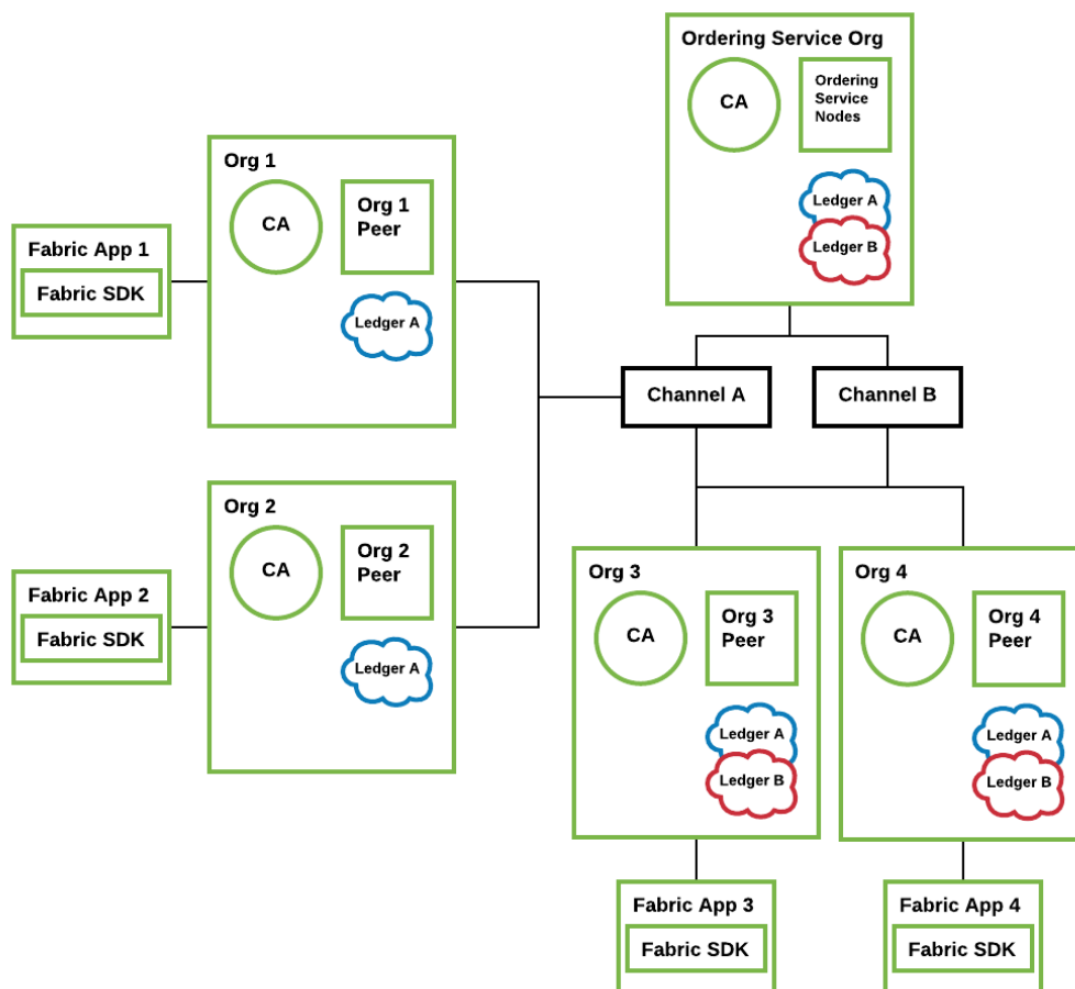
Fig.1: An example Fabric blockchain network with four organizations. The ordering service has ordering nodes for ordering and distributing blocks on each of the channels defined under the ordering service. Channel A includes all four organizations, while channel B includes only Org 3 and Org 4. Authenticated client applications can send calls to their associated peers on the network.
