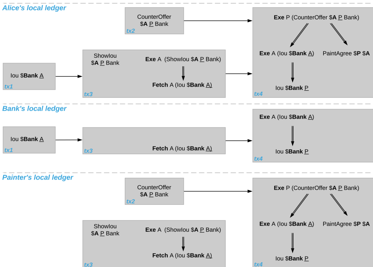
Fig. 4: Projections of the split counteroffer causality graph .
