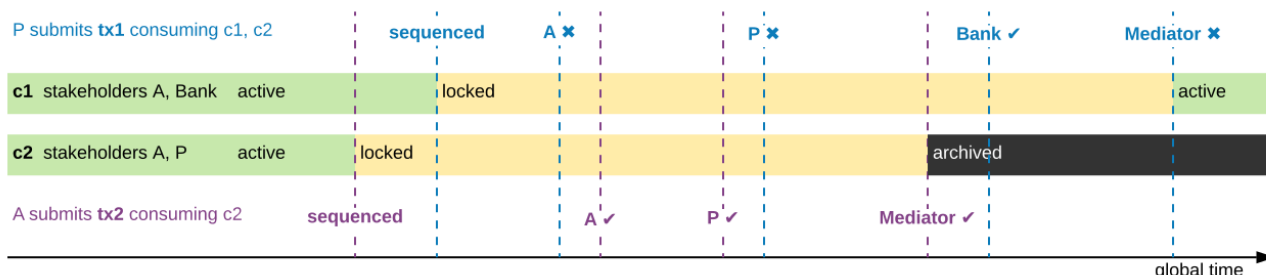
Fig. 5: Transaction tx2 is now submitted before tx1. The consumed contract c1 remains locked by the rejected transaction until the mediator sends the result message.
